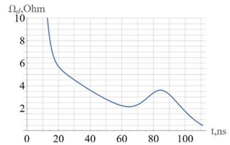
Fig. 2. Typical diode impedance versus time. The active resistance of the diode is equal to the sum of the vacuum gap resistance \Omega_{avc} \approx \frac{1}{U^{1/2}} \frac{d_{acc}^2}{S_{exp}} for the value of the cathode-anode gap equal to d_{acc} and resistance of the plasma conductor \Omega_{pl} \sim I_{pl}(t) .
