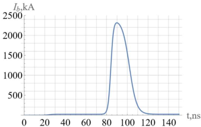
Fig. 4. Characteristic view of the current after leaving the region of the exploding anode (in the region of the return conductor). The effect of charge reset effect in a diode with a virtual cathode is observed [5]. The current amplitude is several times greater than the current amplitude in the diode and in some experiments exceeded 2.5 MA. The current energy for the entire time after the explosion reached 100 kJ, which exceeded the energy (about 30 kJ) contained in the primary storage.
