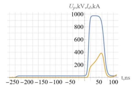
Fig. 3. Characteristic view of the current pulse in the diode, shown together with the high voltage pulse. The characteristic shape of the current pulse is determined by: the time shift of the current pulse maximum from the voltage maximum, the duration of the current pulse, the duration of the leading edge of the current pulse, the amplitude of the current pulse. The maximum value of the electron beam power is about 10^{12} Watts.
