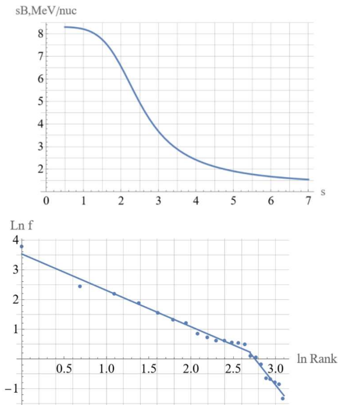
Fig. 6. The dependence of the average binding energy per nucleon on the index of the product spectrum s (top). Typical Zipf-Mandelbrot distribution for the abundance of synthesis products from the experimental results of optical measurements (bottom).
