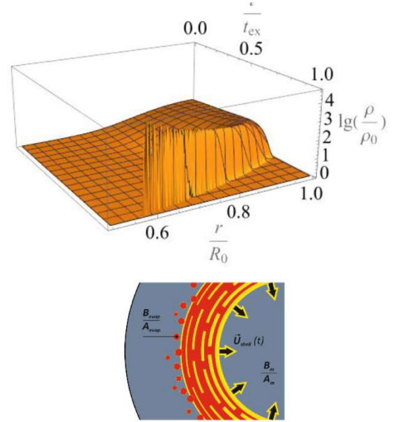
Fig. 5. Nonlinear wave propagating from the surface to the optical center of the target in the implosion blow-up mode. The wave front has a fractal structure [7,13] in a coherently correlated state, through which the substance of the medium is filtered and new nuclei are formed at the trailing wave front. The estimates for density of nonlinear wave were performed in the hydrodynamic approximation using the Lagrangian particle method.
