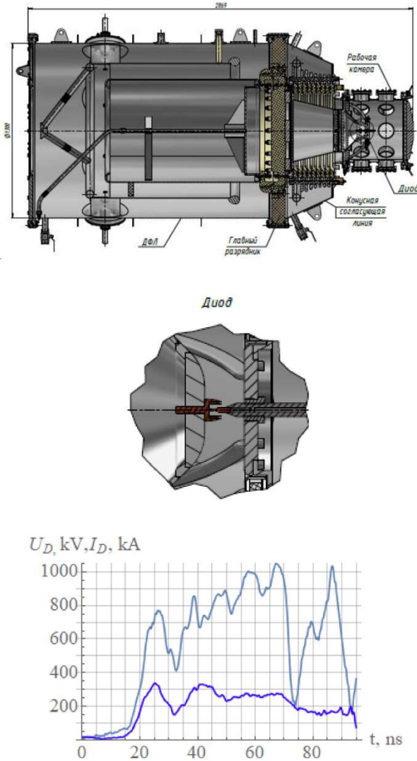
Fig. 10. Sketch of the DFL and diode of the ShAD unit. Typical oscillograms of current (lower curve) in the electron beam and voltage (upper curve) on the diode (experiment number 41317) on the bottom.
