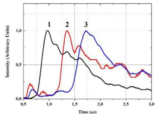
Fig. 11. Intensity of the light registered using a monochromator (NP250-2 M) at different points and calculation of the target explosion products velocities. u_{1-2} = 0,9\text{cm}/0,379 \mu\text{s} = 2,38 \cdot 10^6 \text{cm/s} ; u_{1-3} = 1,8\text{cm}/0,750 \mu\text{s} = 2,40 \cdot 10^6 \text{cm/s} ; u_{2-3} = 0,9\text{cm}/0,371 \mu\text{s} = 2,42 \cdot 10^6 \text{cm/s} .
